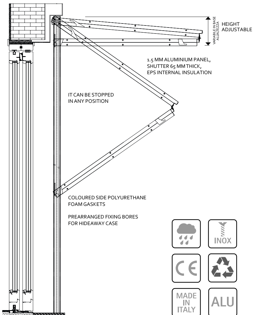
Completely coplanar panels when closed vertically; complete opening by horizontal panels.
